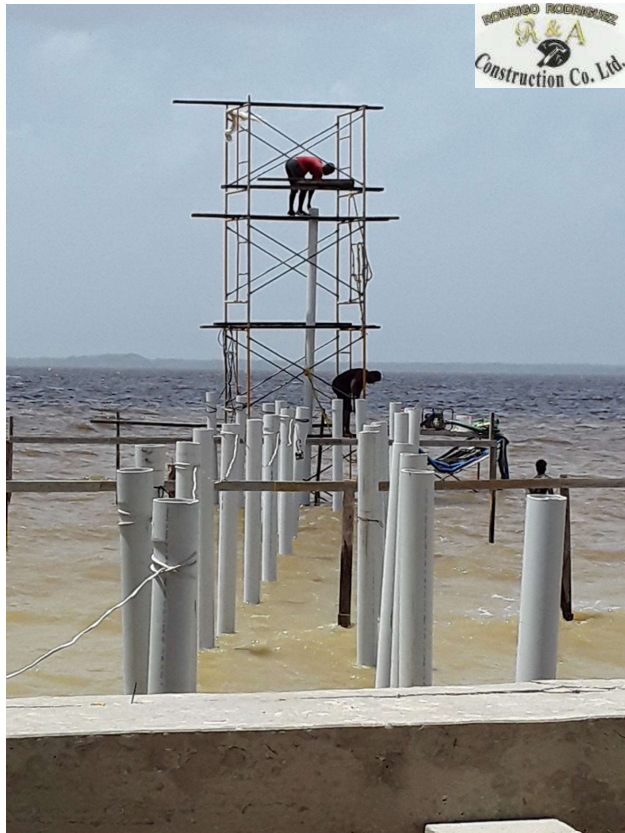
PIER CONSTRUCTION - FINCA SOLANA
