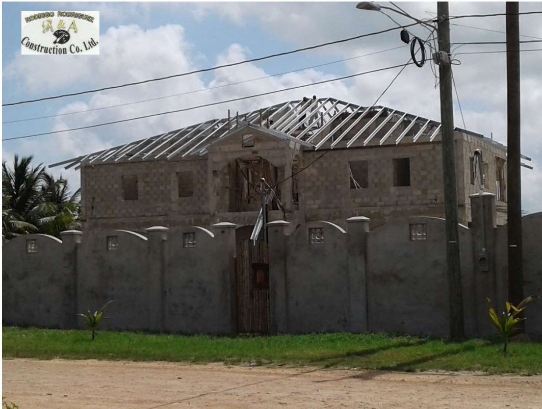
METAL ROOF FRAMING - FINCA SOLANA
